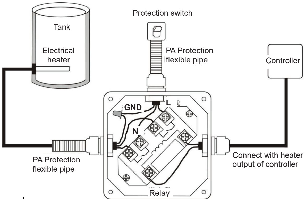
SR802 connection diagram:
